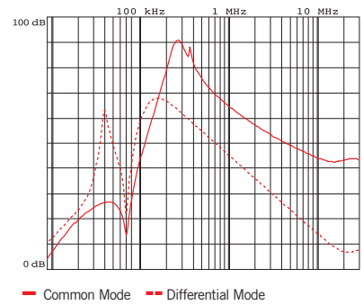
Typical attenuation 7A – 400A
